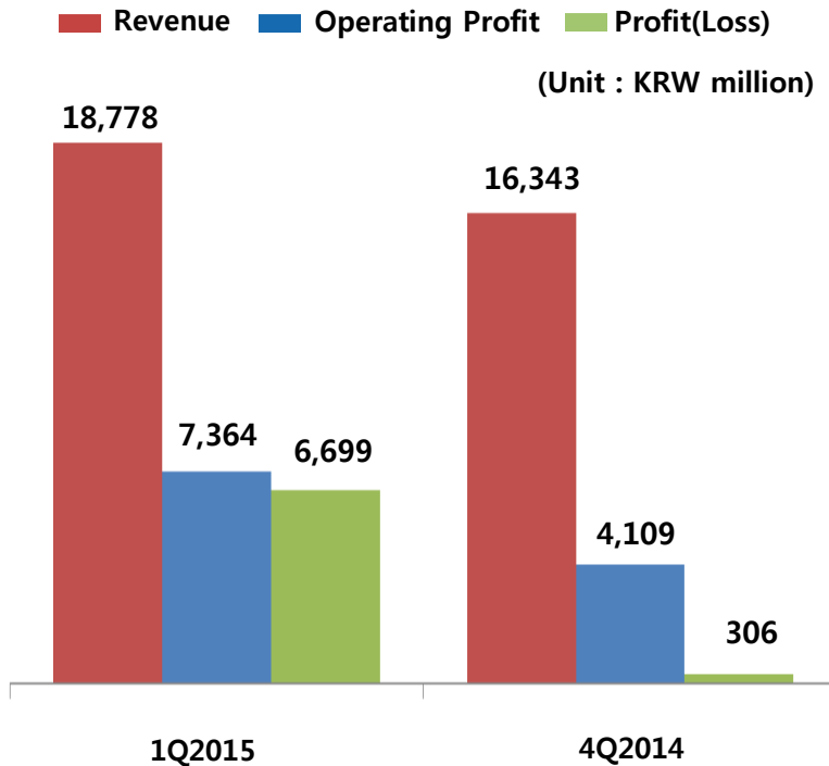
QoQ (Parent)
